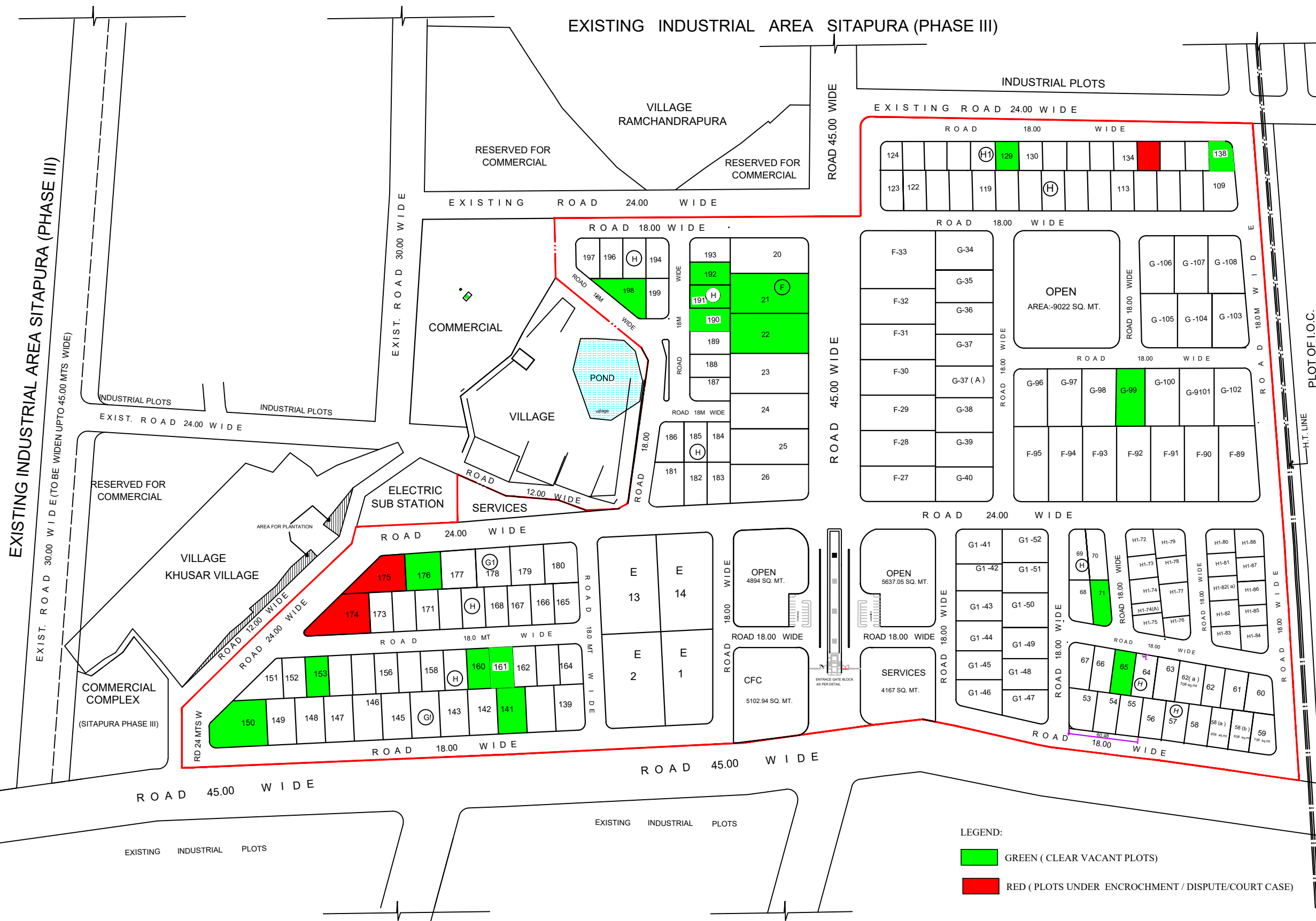
LAYOUT PLAN OF SPECIAL ECONOMIC ZONE - II
