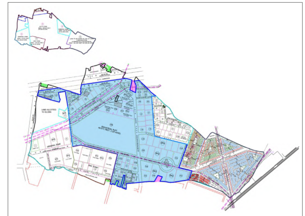
LAYOUT PLAN OF AUTO ZONE, SALARPUR INDUSTRIAL AREA (BHIWADI REGION)
